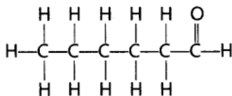
Hexanal ( \text{C}_5\text{H}_{11}\text{CHO} )
