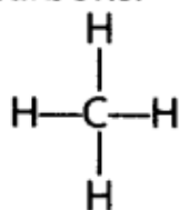
Methane (Saturated hydrocarbon)
