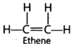
(Unsaturated hydrocarbon)
